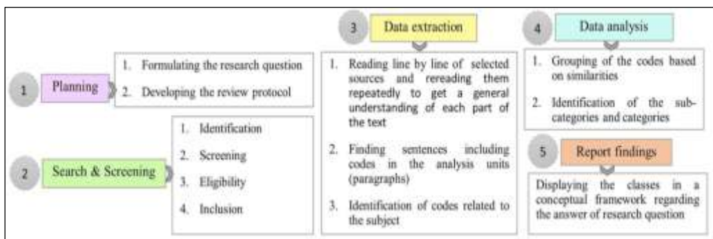
Figure 1. Research process
